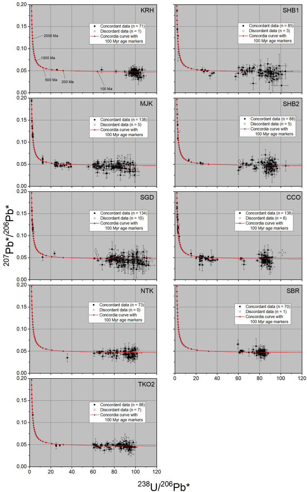
Appendix 4. Tera-Wasserburg diagrams of U–Pb ages for zircons from all nine sandstone samples.
