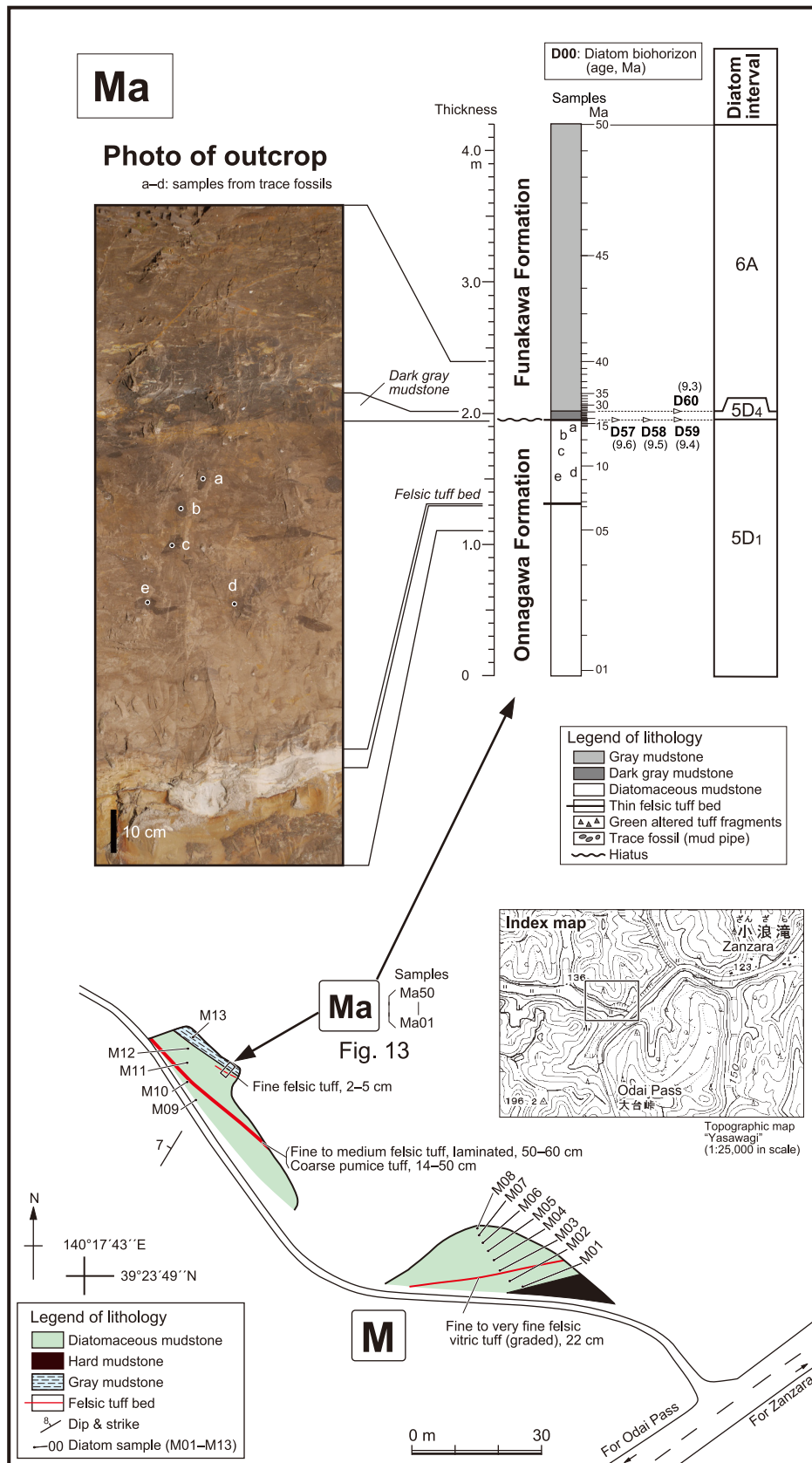
Fig. A6 Route map around stratigraphic section Ma (Fig. 13), to the west of Zanzara, Nangai district, Daisen City. Location of the route map is shown in Fig. A3.
