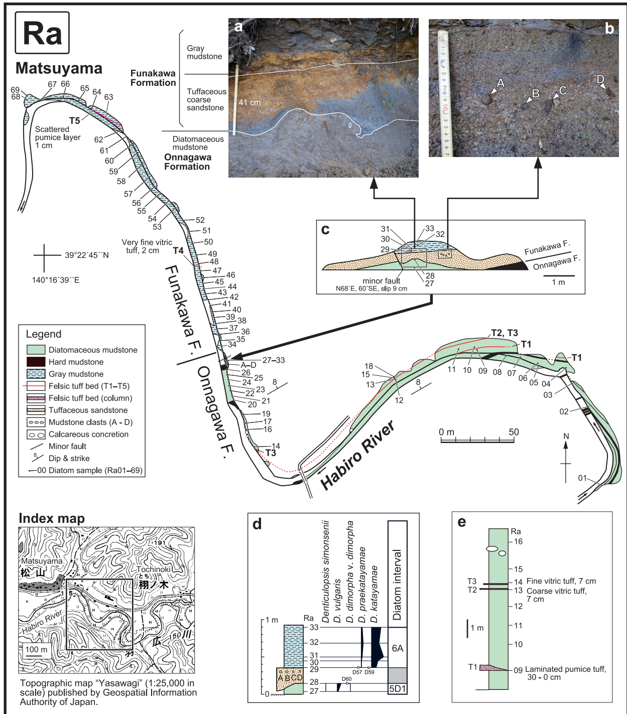
Fig. A5 Route map of the Matsuyama section (Section Ra, Fig. 10) in Matsuyama, Habiro, Ouchi district, Yuri-Honjo City, showing localities of samples Ra01–69 with samples A–D (mudstone clasts in tuffaceous sandstone bed of the basal part of the Funakawa Formation). Location of the route map is shown in Fig. A4.
